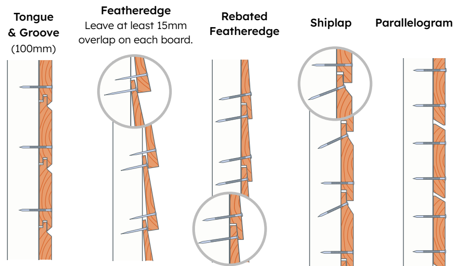
Tongue and Groove profile cladding board - fit with the tongue pointing upwards
